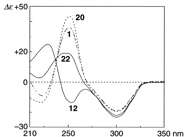
Figure 1. CD spectra of callystatin A ( 1 ) and 10- epi ( 12 ), 5- epi ( 20 ), and 10-demethyl ( 22 ) analogues in MeOH.
