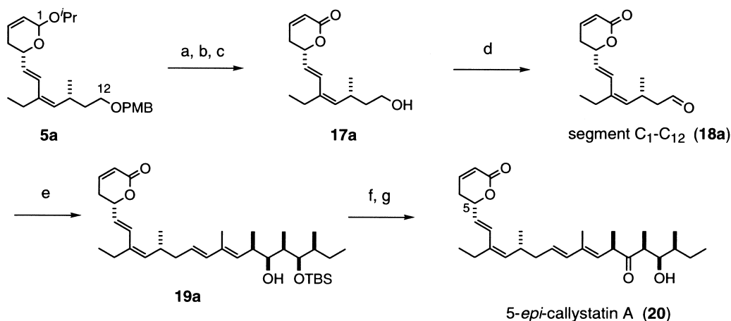
Scheme 3. Reagents and conditions: (a) Dowex HCR-W2, acetone: \text{H}_2\text{O} (5:1), 40^\circ\text{C} ; (b) \text{Ag}_2\text{CO}_3 –Celite, PhH, 50^\circ\text{C} , two steps 91%; (c) DDQ, \text{CH}_2\text{Cl}_2 : n\text{BuOH} :pH 6.9 phosphate buffer (90:1:9), 91%; (d) Dess–Martin periodinane, \text{CH}_2\text{Cl}_2 ; (e) 10 , \text{LiCH}_2\text{S}(\text{O})\text{CH}_3 , toluene, -20^\circ\text{C} , two steps 62%; (f) Dess–Martin periodinane, \text{CH}_2\text{Cl}_2 ; (g) HF:Py (5:1), THF, two steps 90%.
