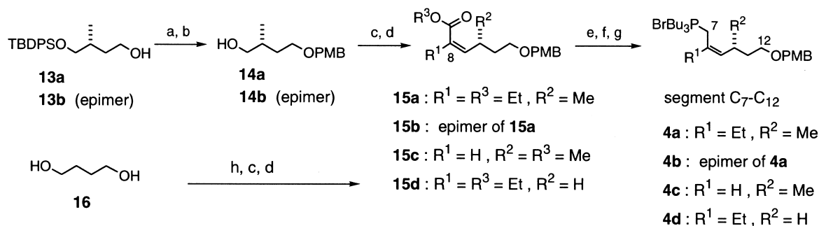
Scheme 2. Reagents and conditions: (a) PMBBBr, NaH, THF, 96%; (b) n\text{Bu}_4\text{NF} , THF, 97%; (c) (\text{COCl})_2 , DMSO, \text{Et}_3\text{N} , \text{CH}_2\text{Cl}_2 ; (d) \text{R}^3\text{OCOCH}(\text{R}^1)\text{PO}(\text{OCH}_2\text{CF}_3)_2 , \text{KN}(\text{SiMe}_3)_2 , 18-crown-6, THF, -78-0^\circ\text{C} , 15a : two steps 92% ( Z:E=12:1 ), 15c : two steps quant. ( Z:E=7.7:1 ), 15d : two steps 95% ( Z:E=5:1 ); (e) DIBAL-H, \text{CH}_2\text{Cl}_2 , -78^\circ\text{C} ; (f) \text{CBr}_4 , \text{PPh}_3 , 2,6-lutidine, \text{CH}_3\text{CN} ; (g) \text{Bu}_3\text{P} , \text{CH}_3\text{CN} , three steps 4a : 92%, 4c : 85%, 4d : 98%; (h) KH, PMBCl, THF, 77%.
