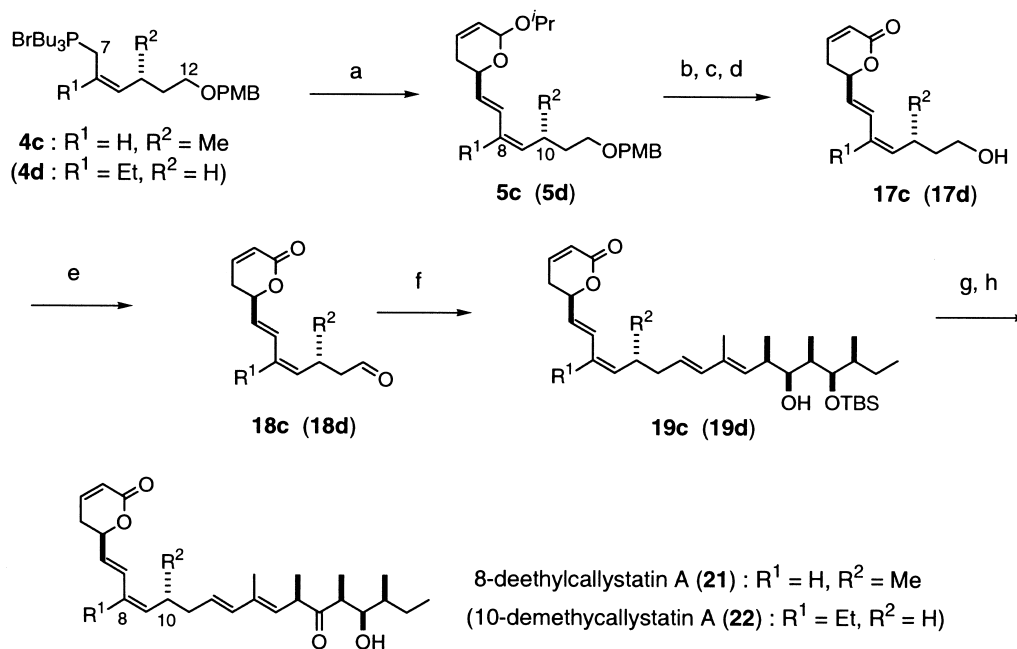
Scheme 4. Reagents and conditions: (a) 3a , LiCH_2S(O)CH_3 , toluene, -20^\circ C ; 5c : 75%; 5d : 81%; (b) Dowex; HCR-W2, acetone:H 2 O (5:1), 40^\circ C ; (c) Ag_2CO_3 –Celite, PhH, 50^\circ C ; (d) DDQ, CH_2Cl_2 : t BuOH:pH 6.9 phosphate buffer (90:1:9); 17c : three steps 81%, 17d : three steps 76%; (e) Dess–Martin periodinane, CH_2Cl_2 ; (f) 10 , LiCH_2S(O)CH_3 , toluene, -20^\circ C , 19c : two steps 66%, 19d : two steps 65%; (g) Dess–Martin periodinane, CH_2Cl_2 ; (h) HF:Py (5:1), THF; 21 : two steps 85%, 22 : two steps 80%.
