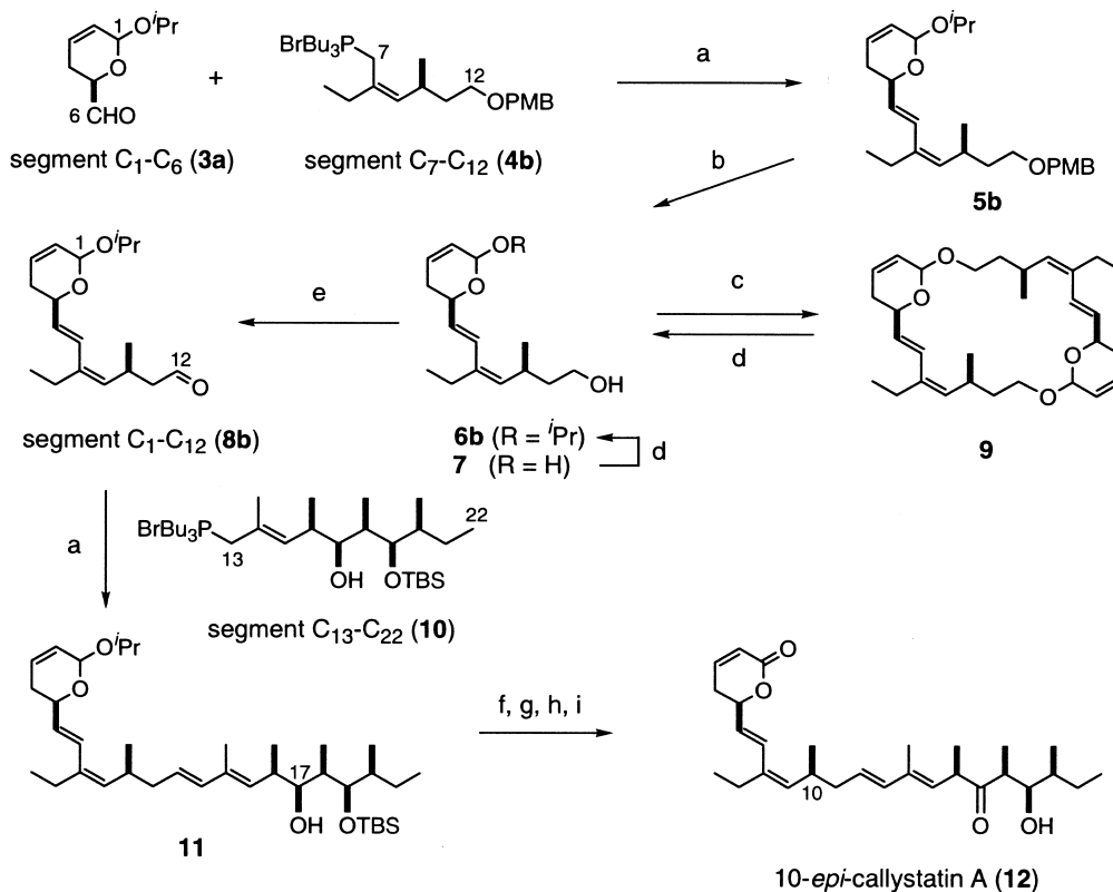
Scheme 1. Reagents and conditions: (a) \text{LiCH}_2\text{S}(\text{O})\text{CH}_3 , toluene, -78^\circ\text{C} , rt, 5b : 72% from 4b , 11 : 71% from 6b ; (b) DDQ, \text{CH}_2\text{Cl}_2 : 0.5% aq \text{NaHCO}_3 (9:1), 82%; (c) \text{SiO}_2 column chromatography; (d) PPTS, i\text{PrOH} , 72%; (e) (\text{COCl})_2 , DMSO, \text{Et}_3\text{N} , \text{CH}_2\text{Cl}_2 , -78^\circ\text{C} ; (f) TPAP, NMO, \text{CH}_2\text{Cl}_2 ; (g) Dowex HCR-W2, acetone: \text{H}_2\text{O} (5:1), 40^\circ\text{C} ; (h) \text{Ag}_2\text{CO}_3\text{--Celite} , \text{PhH} , 50^\circ\text{C} , three steps 65%; (i) HF:Py (5:1), THF, 90%.
